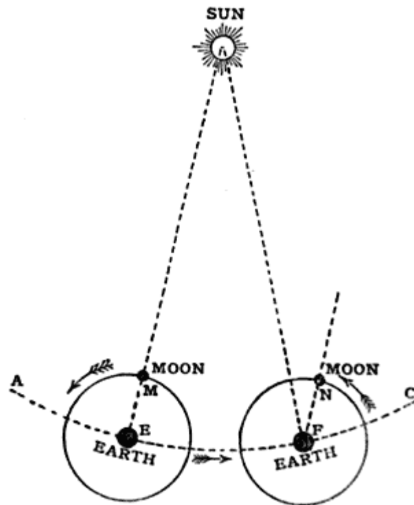
Fig. 2. — Revolution of the Moon round the Earth.
