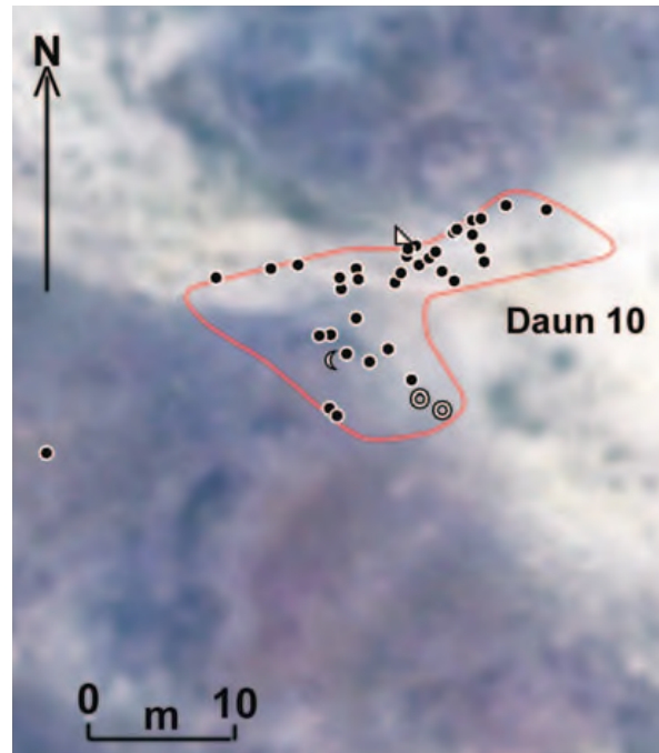
Fig. 10. Daun: shell midden 10: distribution map of chipped stone artefacts (dots), lunate (moon-like symbol), chalcedony fragment (triangle), and coarse ground stones (circles) (drawing C. Franco)
