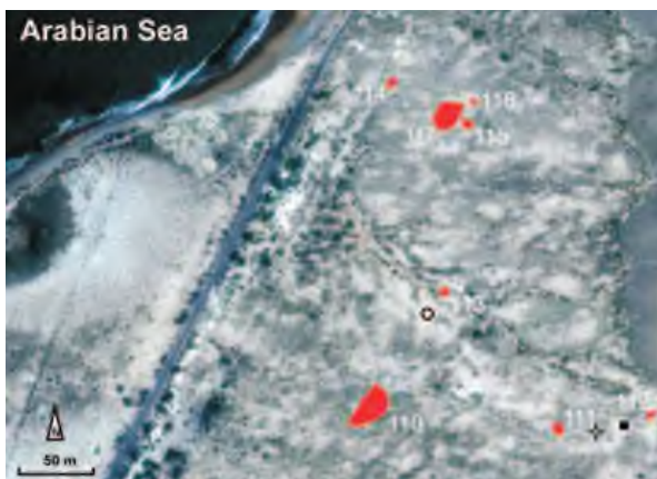
Fig. 3. Daun: distribution map of the shell middens 110–117, along the beach south of the bay: net-sinker (star), quern (circle), core (square) (drawing C. Franco)
