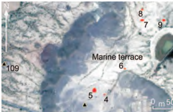
Fig. 2. Daun: distribution map of the shell middens 4–9 on the marine terrace south of the bay. The triangle 109 mark, the point where a quartzite side scarp was found (drawing C. Franco)
