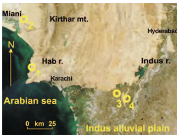
Fig. 16. Distribution map of the radiocarbon-dated 8 th and 7 th millennium BP shell middens of Las Bela and Lower Sindh: 1) Daun, 2) Lake Siranda, 3) Tharro Hills, 4) Makli Hills (drawing P. Biagi)
