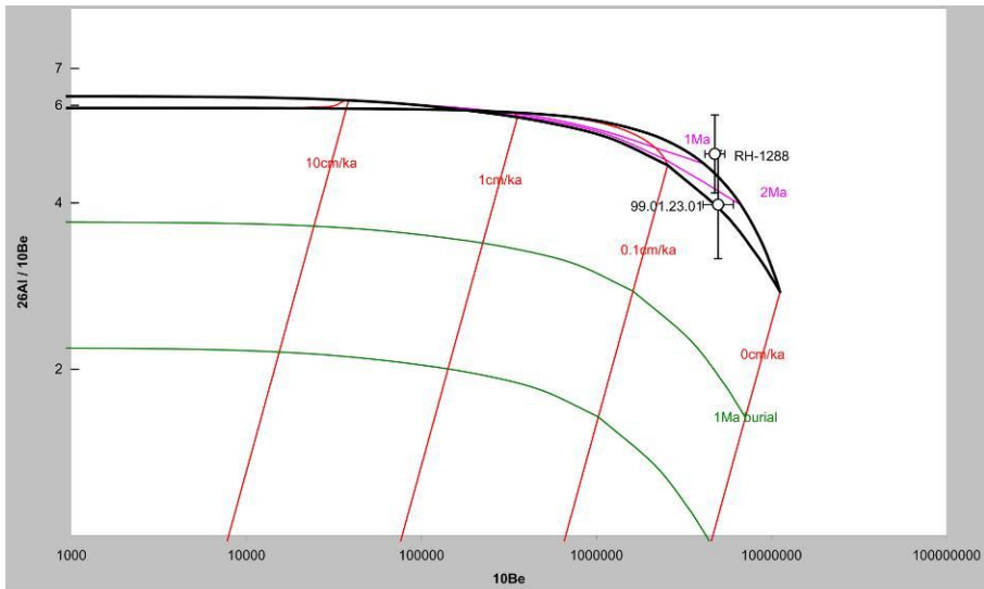
Fig. 43: Results of the TCNs analyses performed on two Rohri Hills samples. The surface exposure age is of some 1.2 Myr (courtesy of C. Baroni)
