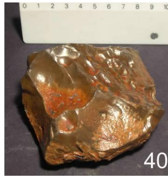
Figs. 39 and 40: Rohri Hills. Eolized, natural flint nodule from Hoban Shah submitted for TCNs analyses (sample 990123.01) (photographs C. Baroni)
